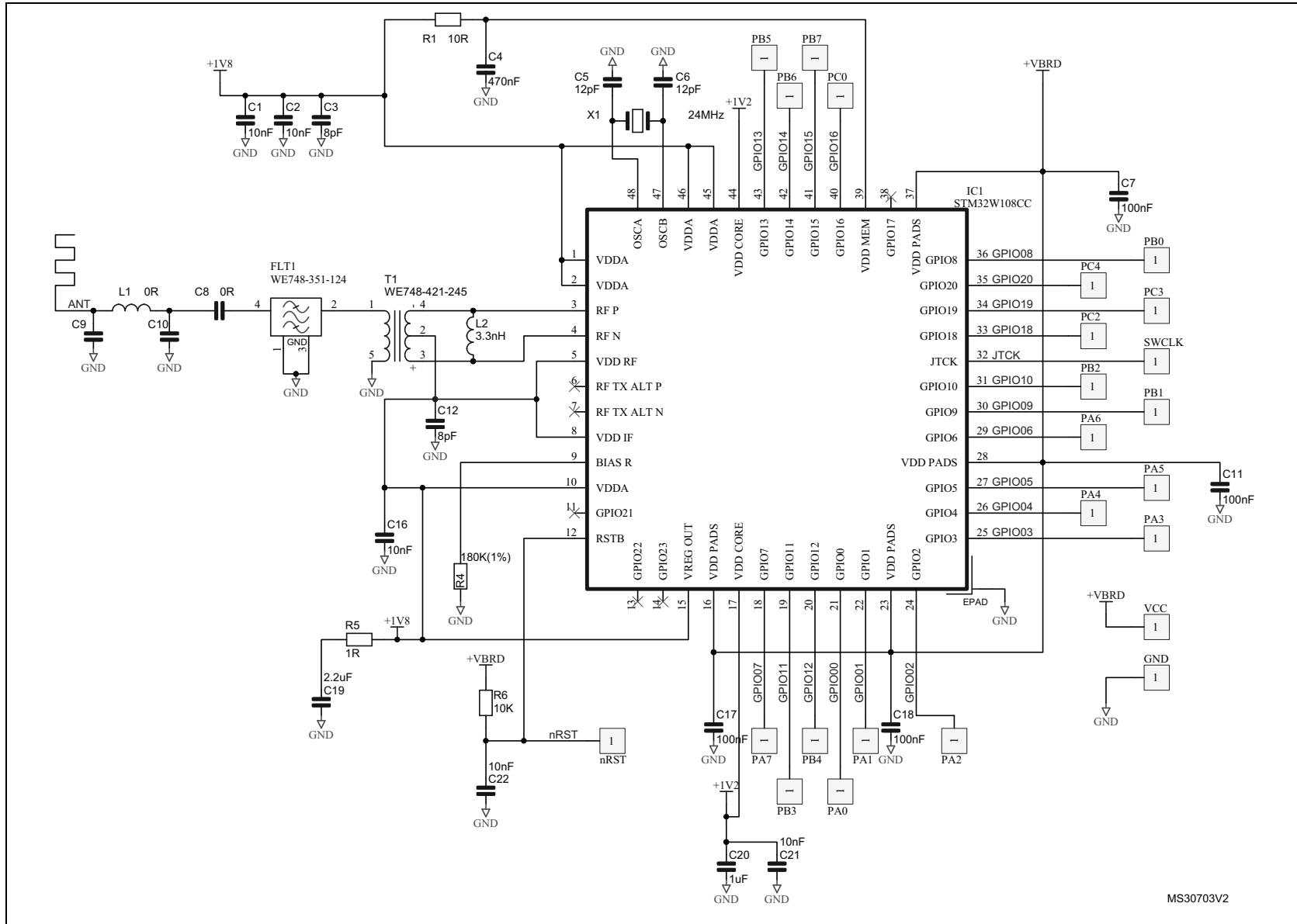
Figure 4. MB953 rev. B
